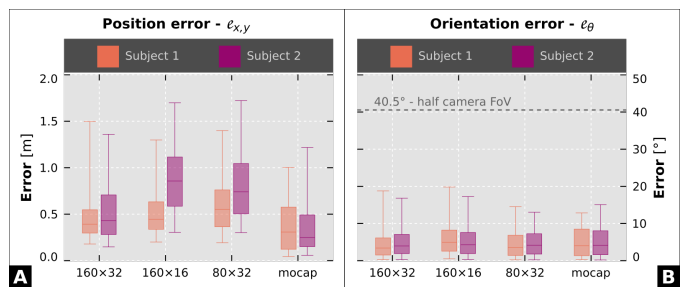
Fig. 16. Distribution of control errors for the two subjects (color), using the proposed models, A) position error and B) orientation error. Boxplot whiskers mark 5^{th} and 95^{th} percentile of data. The dashed line on the right plot marks the half-field of view of the camera ( 40.5^\circ ): when the angular error is smaller, the subject is visible in the frame.
