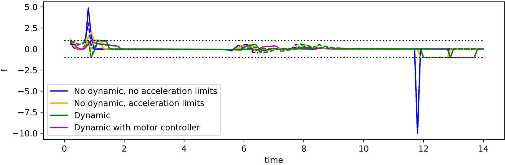
motor forces
